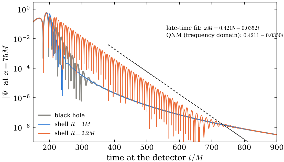
Time-domain simulation: the same pulse ( \ell = 2 , odd) hits each object
